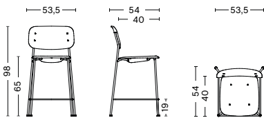
SOFT EDGE 90 LOW WIDTH 53,5 CM DEPTH 54 CM HEIGHT 98 CM SEAT HEIGHT 65 CM SEAT DEPTH 40 CM
