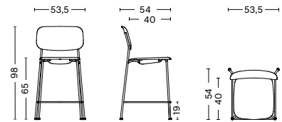
SOFT EDGE 91 LOW | FULL UPHOLSTERY WIDTH 53,5 CM DEPTH 54 CM HEIGHT 98 CM SEAT HEIGHT 65 CM SEAT DEPTH 40 CM
