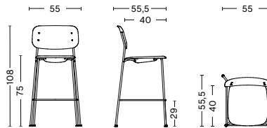
SOFT EDGE 90 HIGH | SEAT UPHOLSTERY WIDTH 55 CM DEPTH 55,5 CM HEIGHT 108 CM SEAT HEIGHT 75 CM SEAT DEPTH 40 CM
