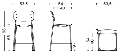
SOFT EDGE 90 LOW | SEAT UPHOLSTERY WIDTH 53,5 CM DEPTH 54 CM HEIGHT 98 CM SEAT HEIGHT 65 CM SEAT DEPTH 40 CM
