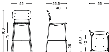
SOFT EDGE 90 HIGH WIDTH 55 CM DEPTH 55,5 CM HEIGHT 108 CM SEAT HEIGHT 75 CM SEAT DEPTH 40 CM
