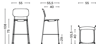
SOFT EDGE 91 HIGH | FULL UPHOLSTERY WIDTH 55 CM DEPTH 55,5 CM HEIGHT 108 CM SEAT HEIGHT 75 CM SEAT DEPTH 40 CM
