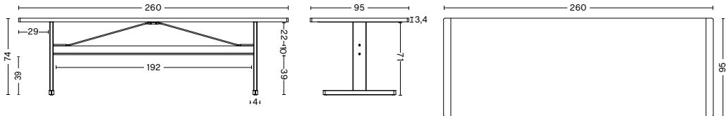
PASSERELLE TABLE | VENEER TABLETOP WIDTH 260 CM | 102.5" DEPTH 95 CM | 37.5" HEIGHT 74 CM | 29.25" CROSSBAR HEIGHT 39 CM | 15.5"
