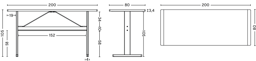
PASSERELLE HIGH TABLE | VENEER TABLETOP WIDTH 200 CM | 78.75" DEPTH 80 CM | 31.5" HEIGHT 105 CM | 41.25" CROSSBAR HEIGHT 58 CM | 22.75"
