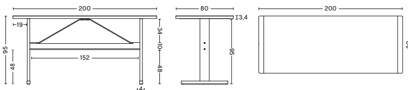
PASSERELLE HIGH TABLE | VENEER TABLETOP WIDTH 200 CM | 78.75" DEPTH 80 CM | 31.5" HEIGHT 95 CM | 37.5" CROSSBAR HEIGHT 48 CM | 19"
