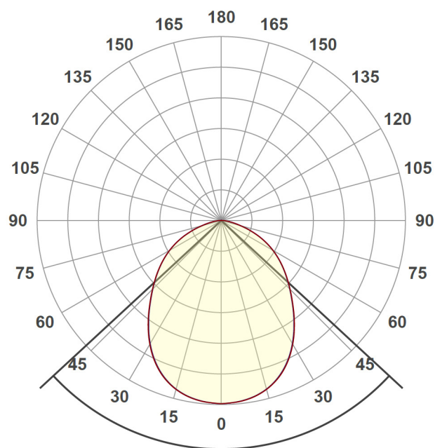
Beam angle: 94° Intensity distribution - Polar
